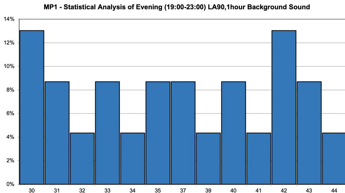
FIGURE 9: STATISTICAL ANALYSIS OF L A90 BACKGROUND – EVENING TIME - MP1
