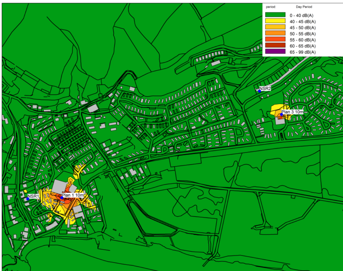
FIGURE 5: EVENING TIME MUSIC SOUND LEVEL NOISE MAP
